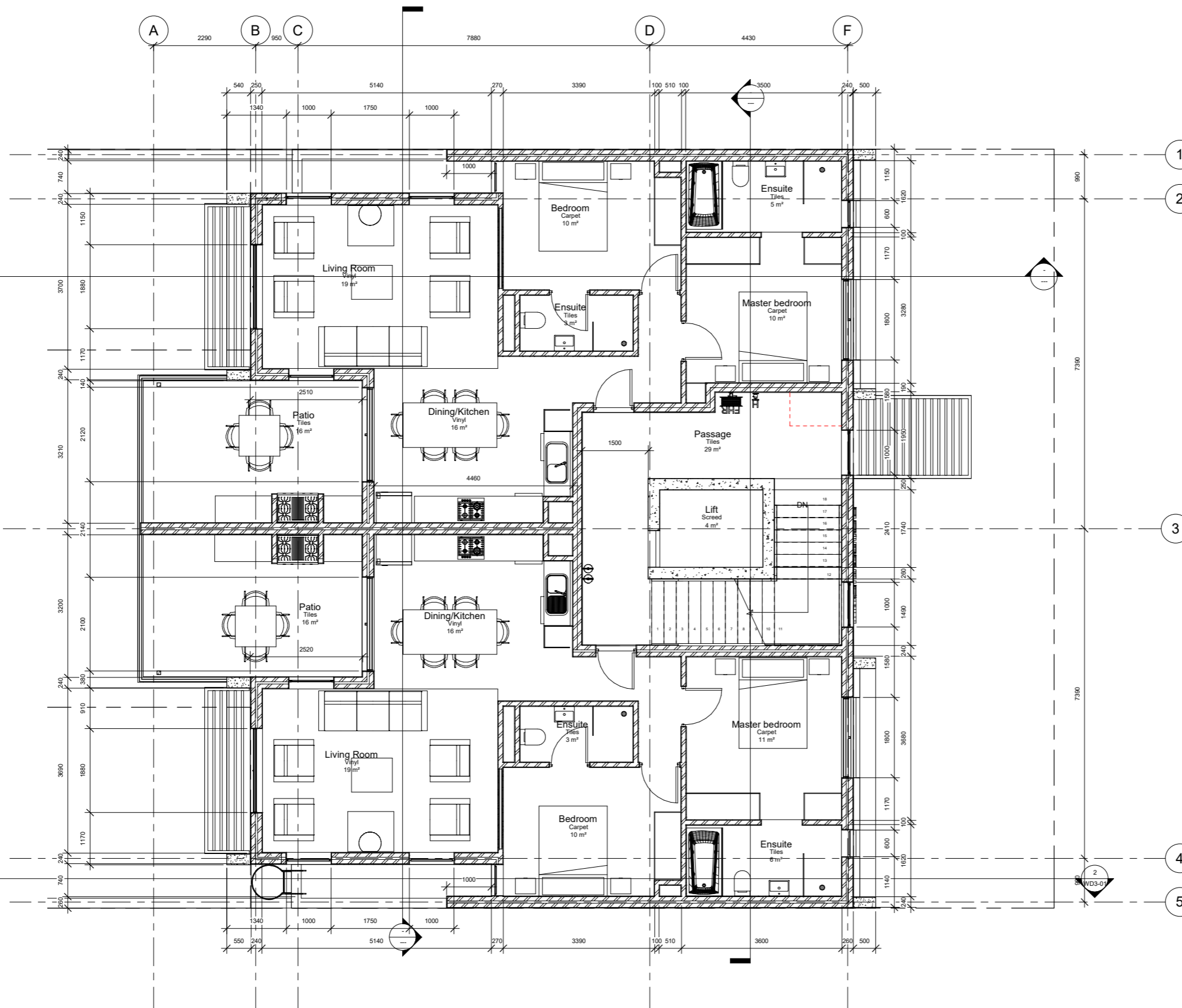
1 2 - First Storey 1: 50
